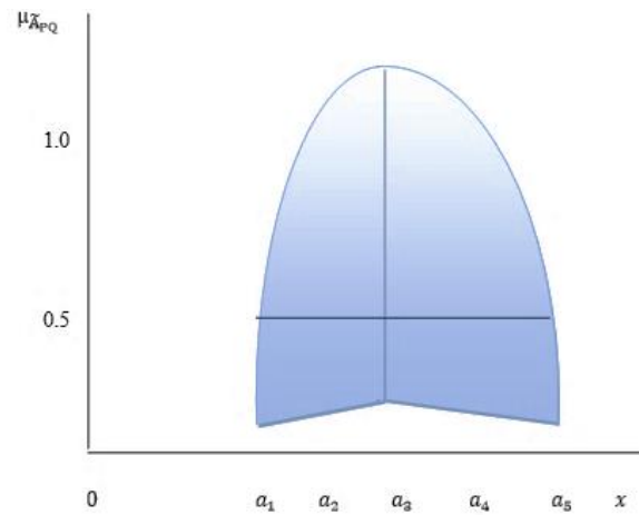
Fig. 1. Graphical representation of a piecewise quadratic fuzzy number.
