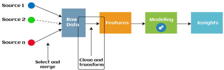
Fig. 4. Feature engineering.
