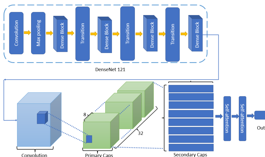
Fig. 1. Proposed Dense Caps (DenseNet-121 and Capsule Net) with self-attention model.
